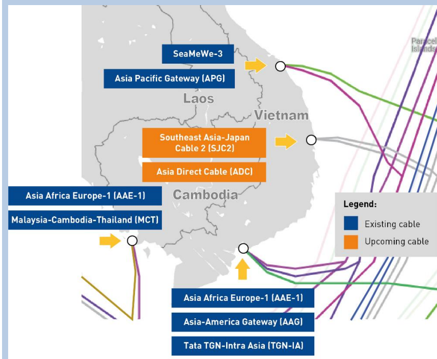
Figure 3.3: Overview of submarine cables connecting to the Indochina region [Source: TeleGeography, Analysys Mason, 2021]
